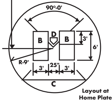
Details of Batter's Box
